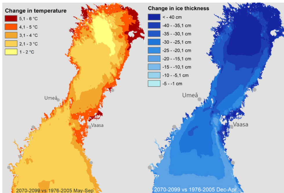
Figure 4.3 (left) change in bottom temperature during May-Sept. (right) change in ice thickness During dec-April. Models created in project ECOnnect.
