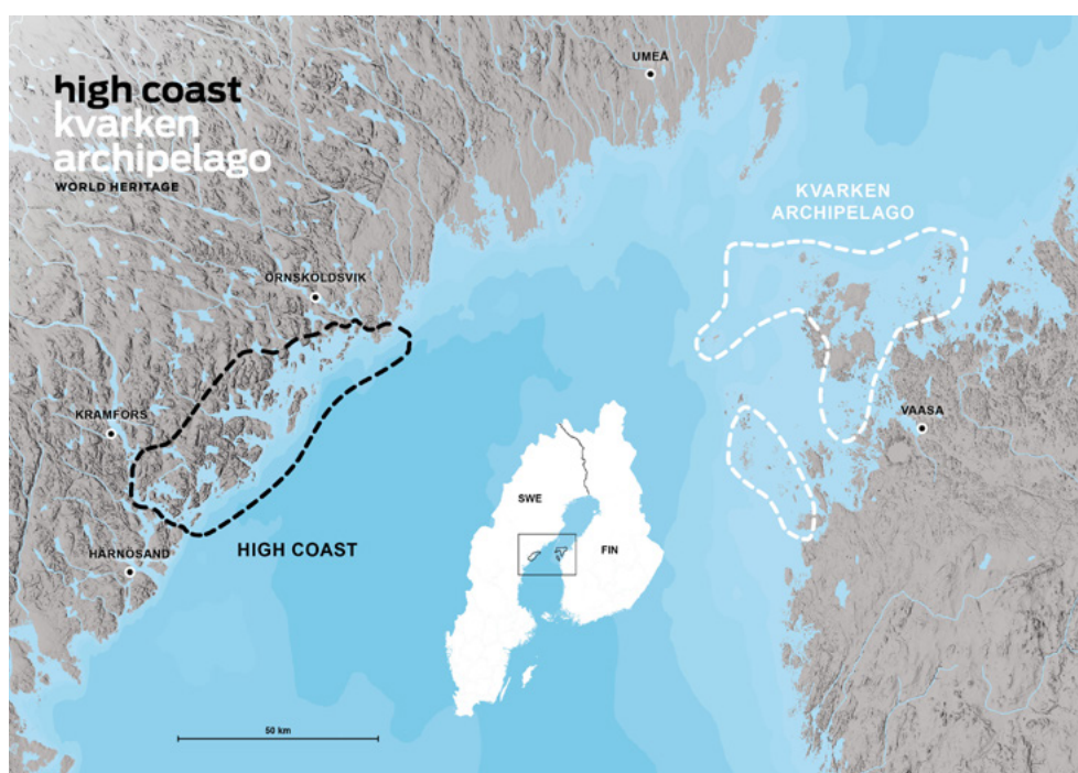
Figure 2.1 - Location of High Coast/Kvarken Archipelago WH property. Map showing the location of the various components in Sweden and Finland of the High Coast/Kvarken Archipelago World Heritage property.
