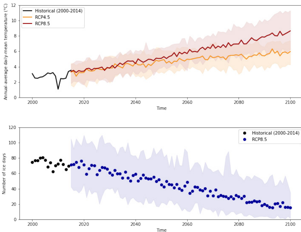
Figure 4.1 (upper) Annual-average temperature for Västernorrland County, historical (2000-2014) and projected (2015-2100) under Representative Concentration Pathway (RCP) 4.5 and 8.5; (lower) Number of days each year for Västernorrland County for which the maximum temperature is projected to be <0^{\circ}\text{C} ('ice days') under RCP8.5.
