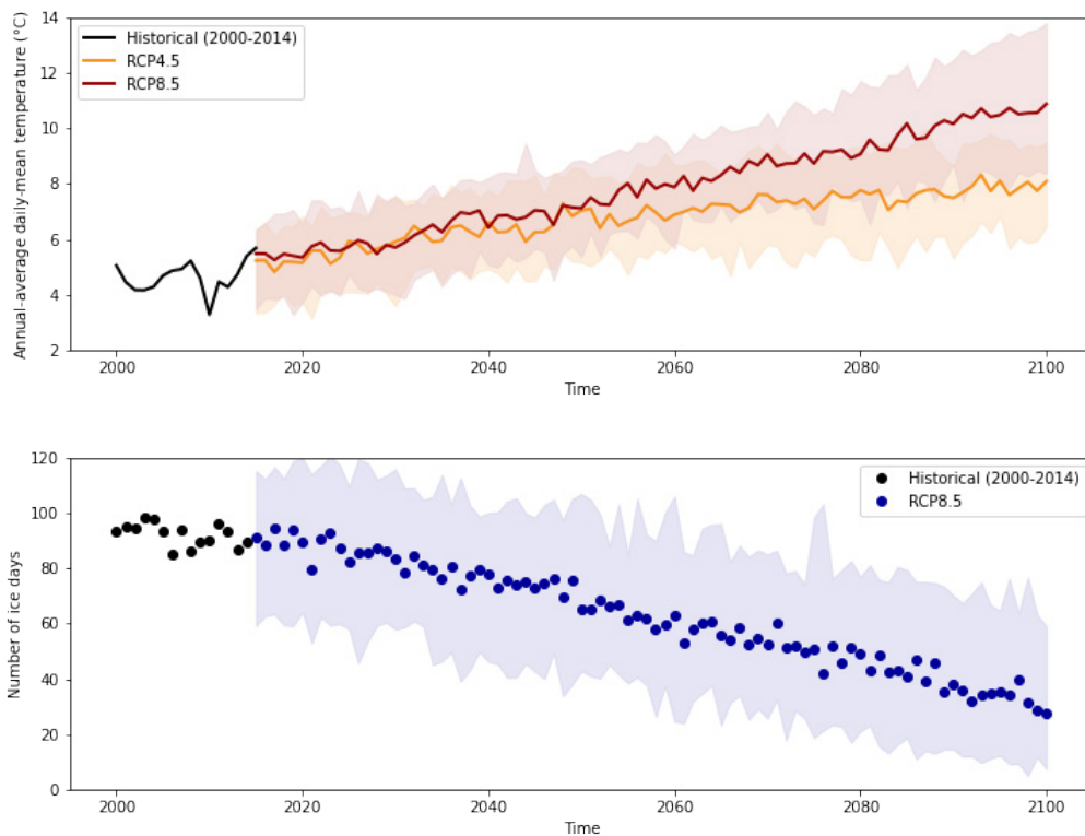
Figure 4.2 (upper) Annual-average temperature for western Finland, historical (2000-2014) and projected (2015-2100) under Representative Concentration Pathway (RCP) 4.5 and 8.5; (lower) Number of days each year for western Finland for which the maximum temperature is projected to be <0^{\circ}\text{C} ('ice days') under RCP8.5.
