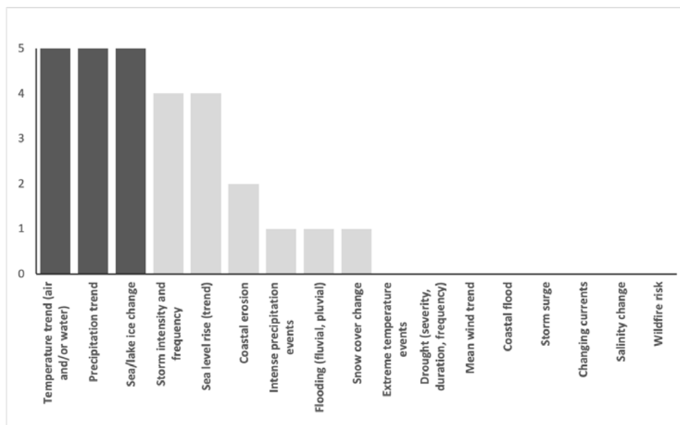
Figure 5.3 Histogram of the number of key values of OUV for High Coast/Kvarken Archipelago for which each of 17 climate stressors were among the top three likely to cause impacts (ca. 2050, high-emissions scenario).
