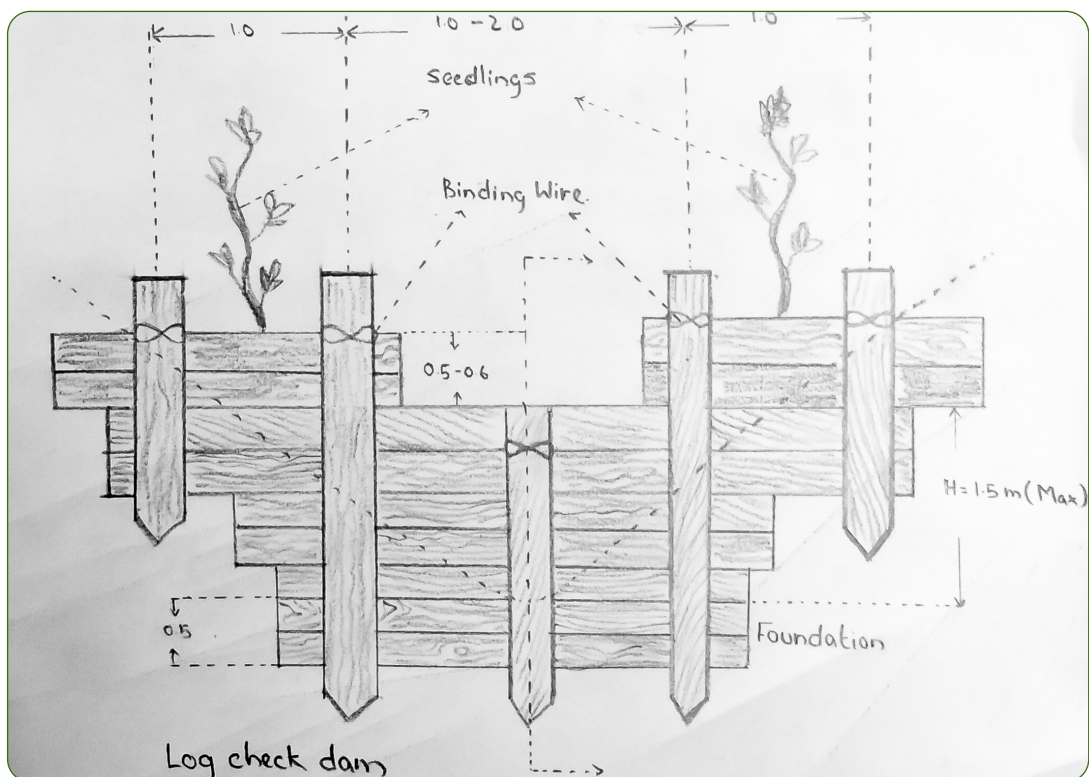
Figure 4.6. Log check dam
