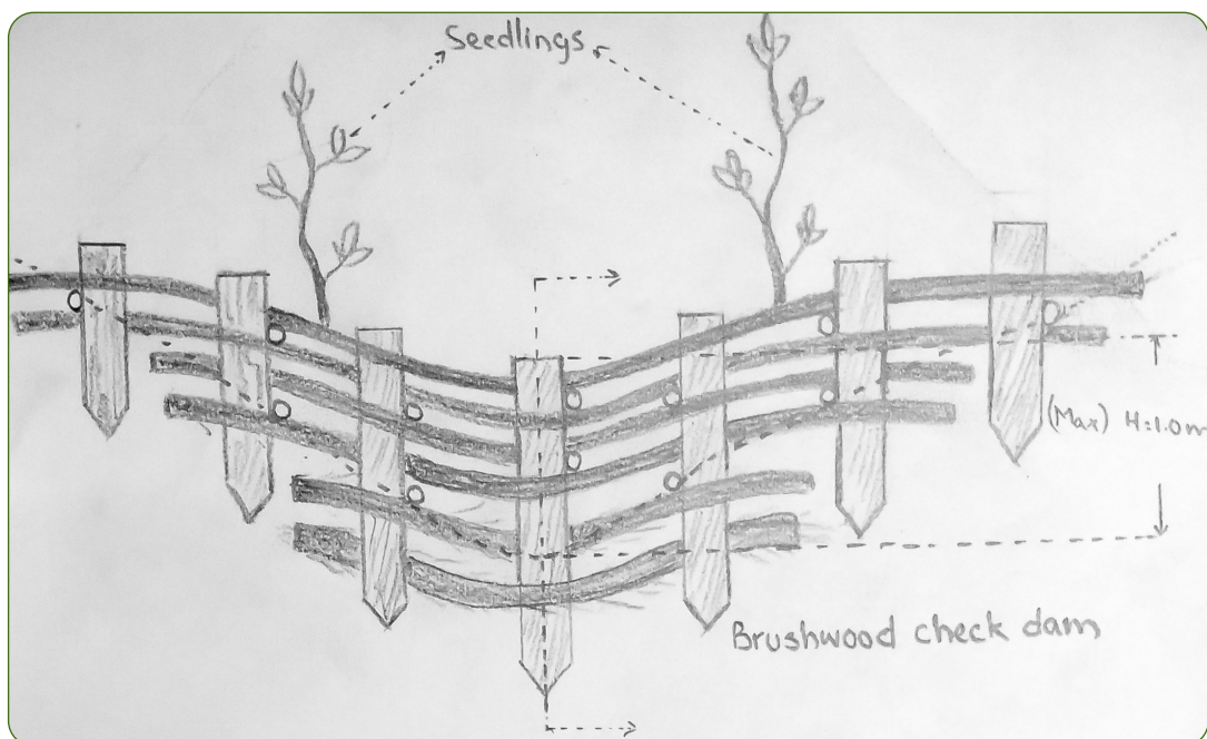
Figure 4.5. Brushwood check dam
